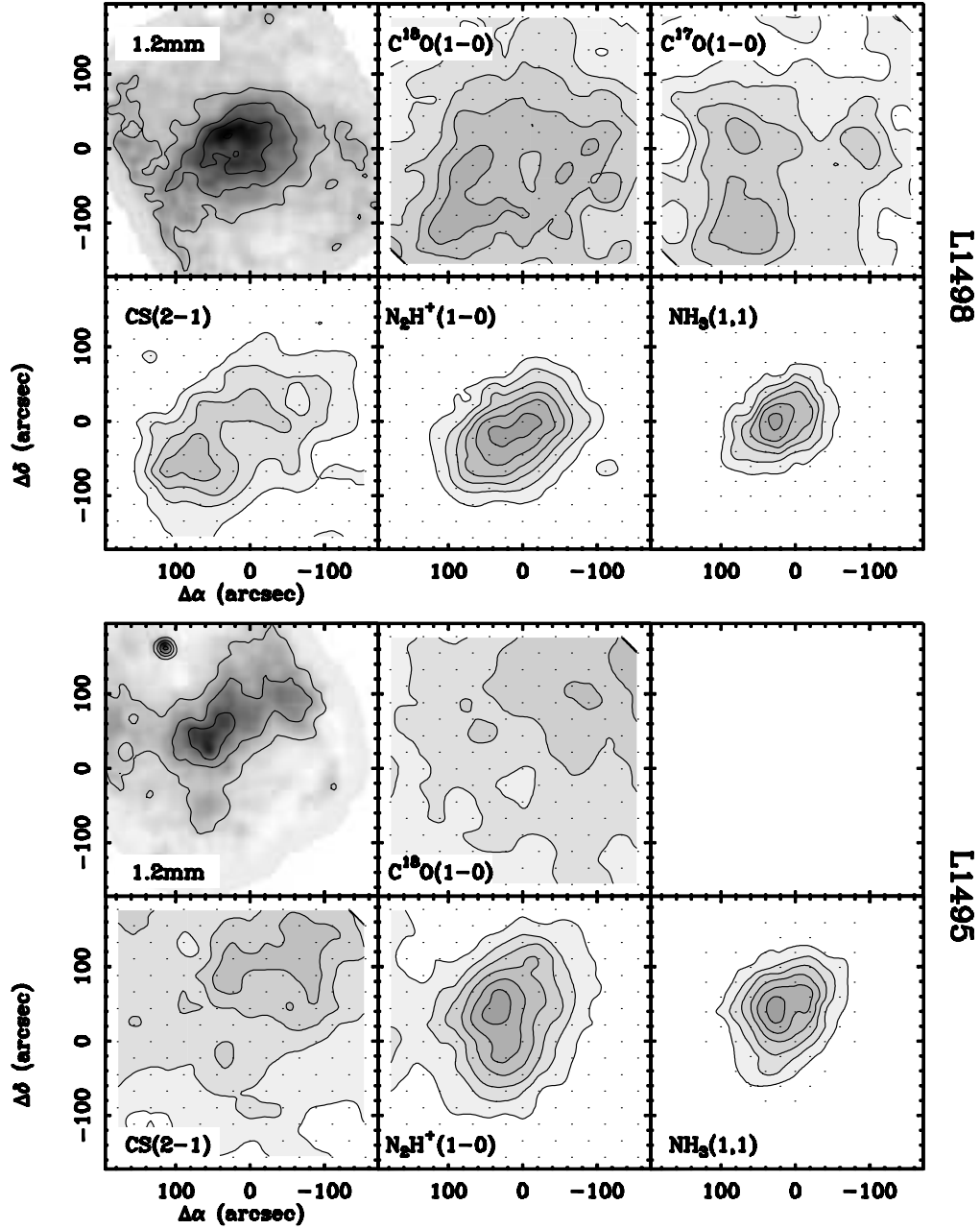
FIG. 1.— Maps of 1.2mm continuum (IRAM 30m telescope), C^{18}O(1-0) , C^{17}O(1-0) , CS(2-1) , N_2H^+(1-0) (FCRAO telescope) and NH_3(1,1) (100m telescope) for L1498, L1495, L1400K, L1517B, and L1544 (L1544 1.2mm continuum map from Ward-Thompson et al. 1999). Central coordinates are given in Table 1. For each map, the first contour and the contour interval are the same. In the 1.2mm maps of L1498, L1495, L1400K, and L1517B, contours start at 5 mJy/11''-beam, although the maps have been convolved to a resolution of 20'', and in the L1544 map, contours start at 20 mJy/13''-beam. The line maps represent integrated intensities including all hyperfine components. The first contour of each map ordered from left to right and from top to bottom are as follows (all in K km s^{-1} , in the main beam temperature scale): L1498 (0.2, 0.075, 0.15, 0.3, 1.5); L1495 (0.3, 0.15, 0.45, 1.5); L1400K (0.2, 0.1, 0.3, 1.0); L1517B (0.2, 0.065, 0.1, 0.3, 1.5), L1544 (0.3, 0.13, 0.15, 0.55, 2.0). Note that the point source to the NE of L1495 in the 1.2mm continuum map is IRAS 04112+2803 (aka CW Tau).
